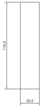
PCB MAX SIZE
